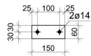
2x (1058) BL10x60x150 S235JR - 1:10
