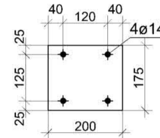
2x (1056) BL10x175x200 S235JR - 1:10
