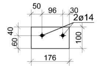
2x (1052) BL10x100x176 S235JR - 1:10
