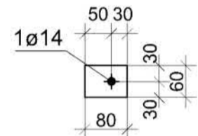
2x (1059) BL10x60x80 S235JR - 1:10
